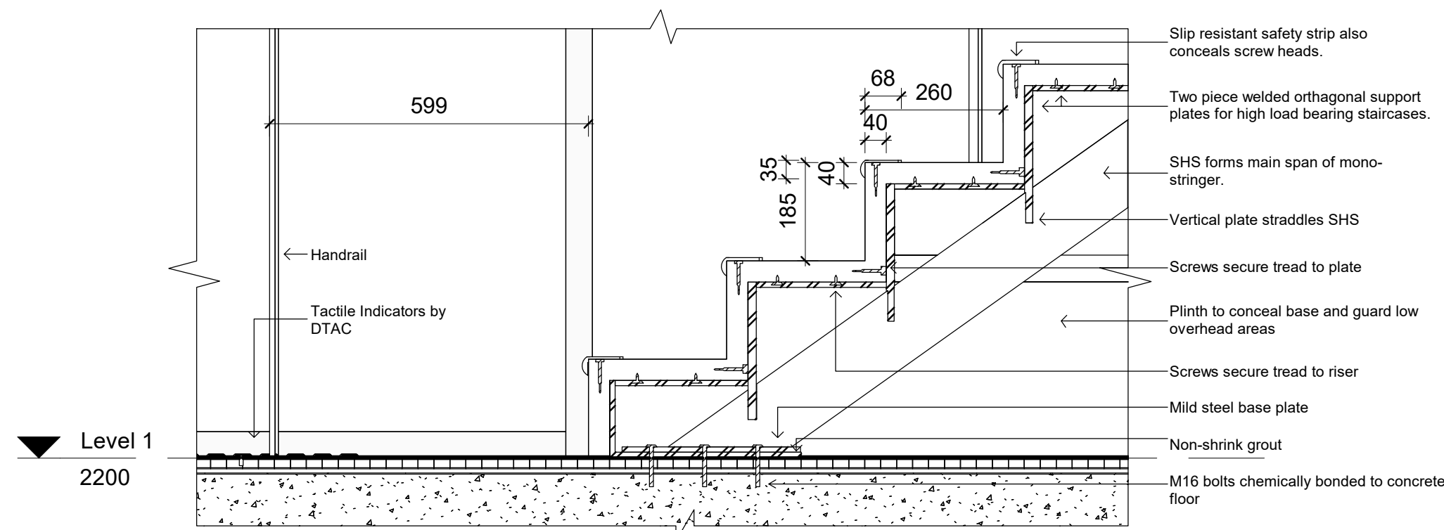
2 Staircase Base Detail 1 : 10
