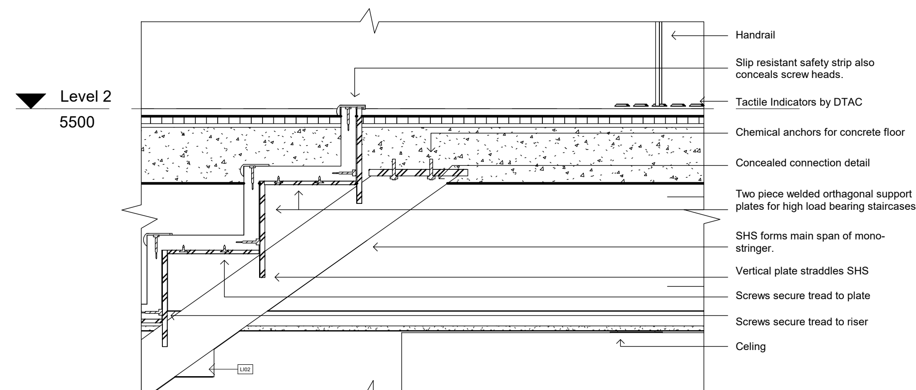
3 Staircase Level 2 Detail 1 : 10
