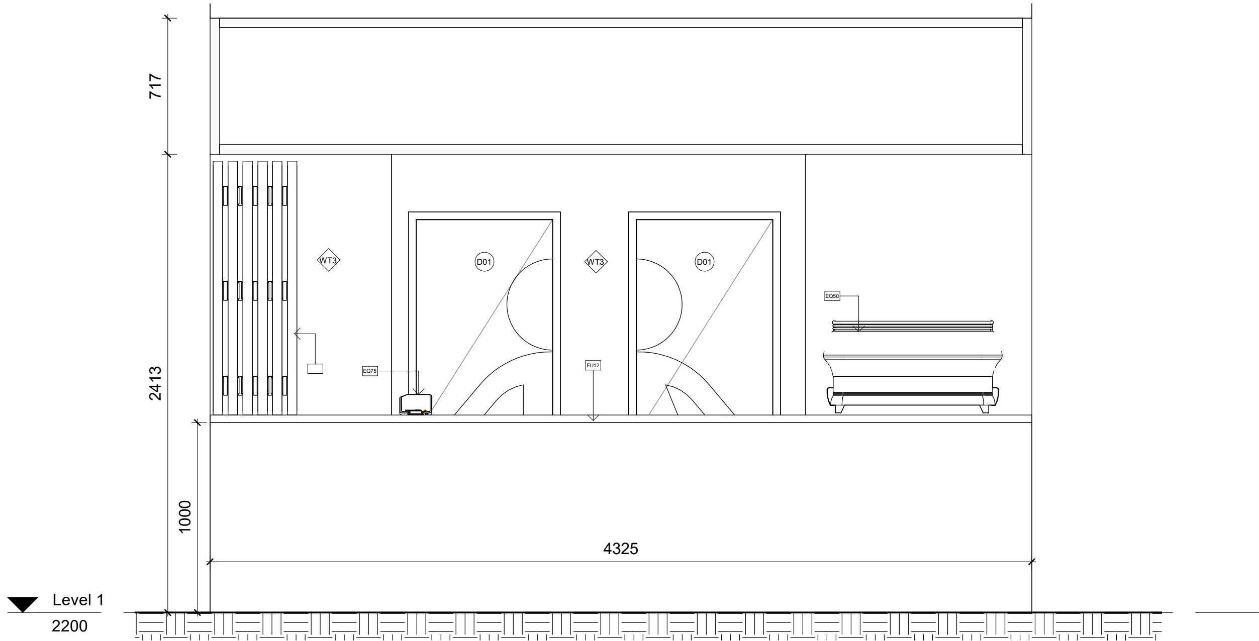
1 Take-Away Bar Section 1 : 20
