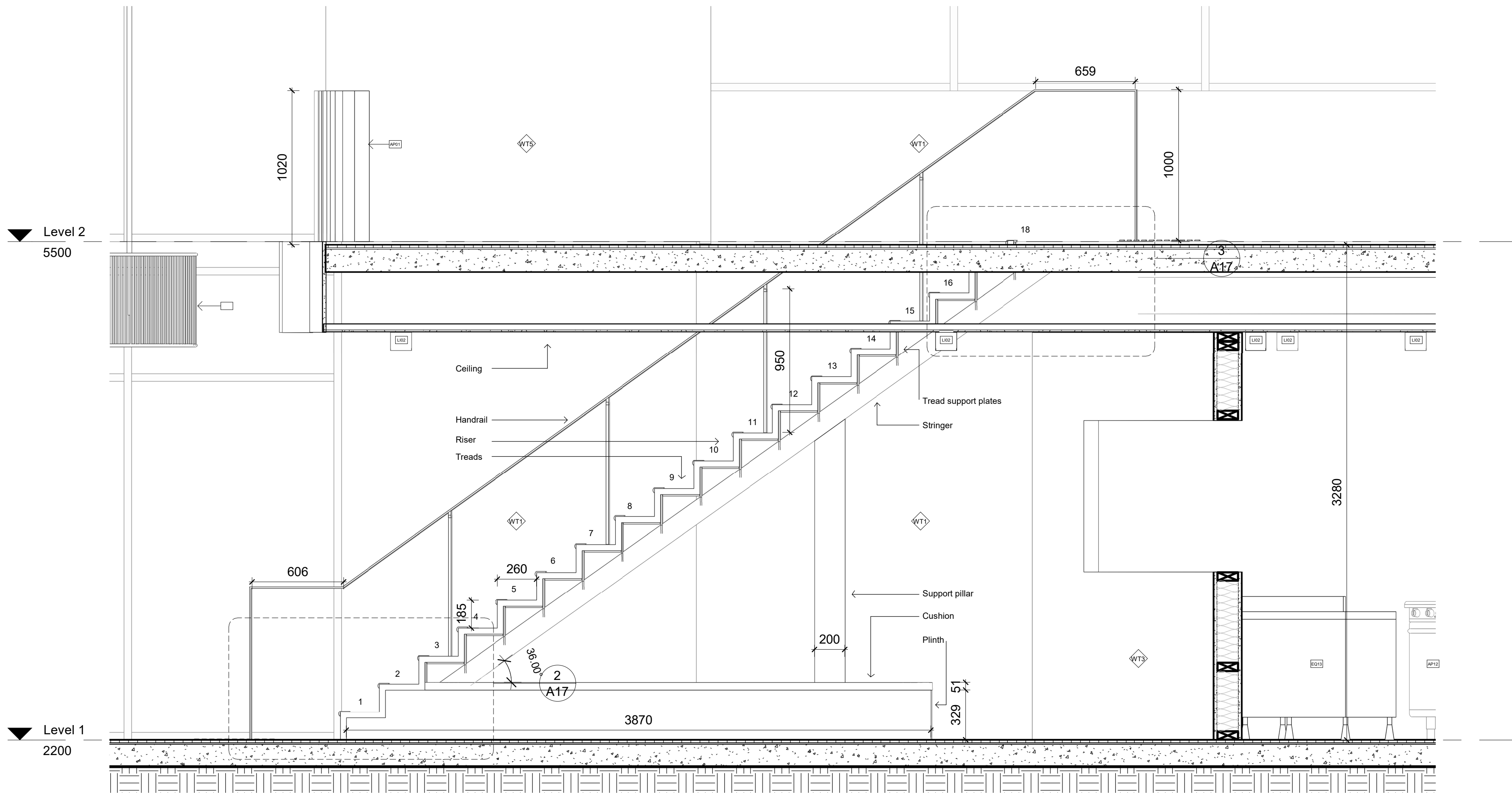
1 Staircase Section 3 1 : 20
